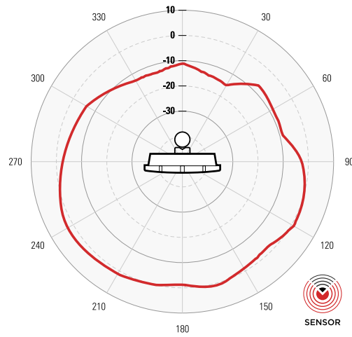
Elevation — 5GHz
