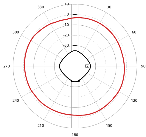
Radio 0 Azimuth — 5GHz
